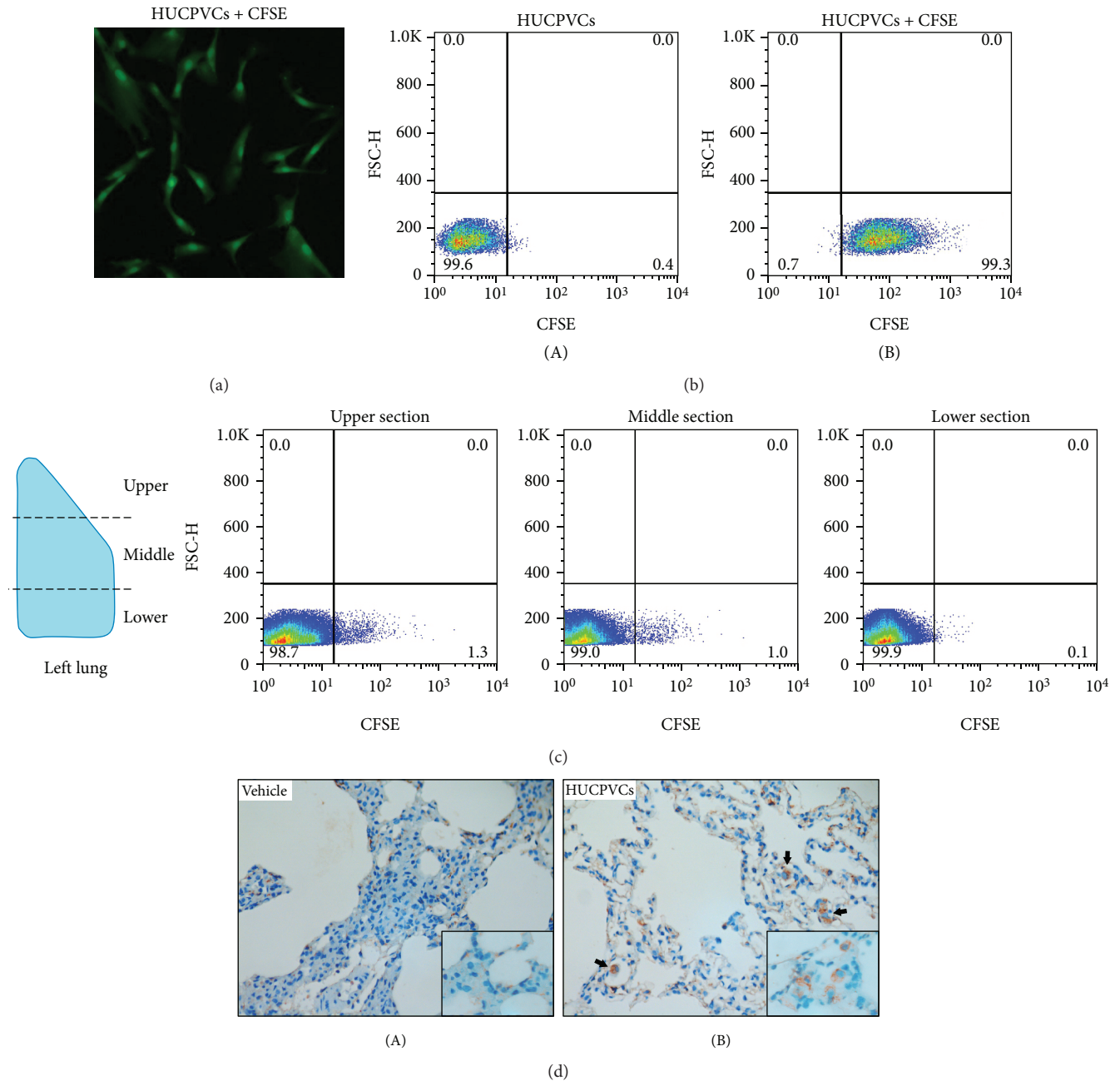
FIGURE 3: Retention of HUCPVCs in the lungs. (a) Representative image of CFSE-labeled HUCPVCs using fluorescence microscopy ( \times 100 original magnification). (b) Flow cytometry analysis of CFSE-labeled HUCPVCs. (A) Dot plot for the unstained control. (B) Dot plot for CFSE-labeled HUCPVCs showing that more than 99% of the cells were positively stained. Data are representative of three independent experiments. (c) Detection of CFSE-labeled HUCPVCs in the lungs by flow cytometry. CFSE-labeled HUCPVCs ( 1 \times 10^6 cells) were administered via the pulmonary artery as described in Materials and Methods (Section 2.2). At the end of the experiment, samples from the upper, middle, and lower sections of the left lung were obtained and analyzed by flow cytometry. Data are representative of three independent experiments. (d) Identification of HUCPVCs in the lungs by immunostaining against human vimentin. Representative images of lung tissue sections obtained at the end of the perfusion from the lungs receiving infusion of vehicle (A) or HUCPVCs (B) at \times 400 original magnification (inset: \times 1000 original magnification). Black arrows indicate vimentin-positive cells. Please note that vimentin-positive cells show a diffuse cytoplasmic staining.
