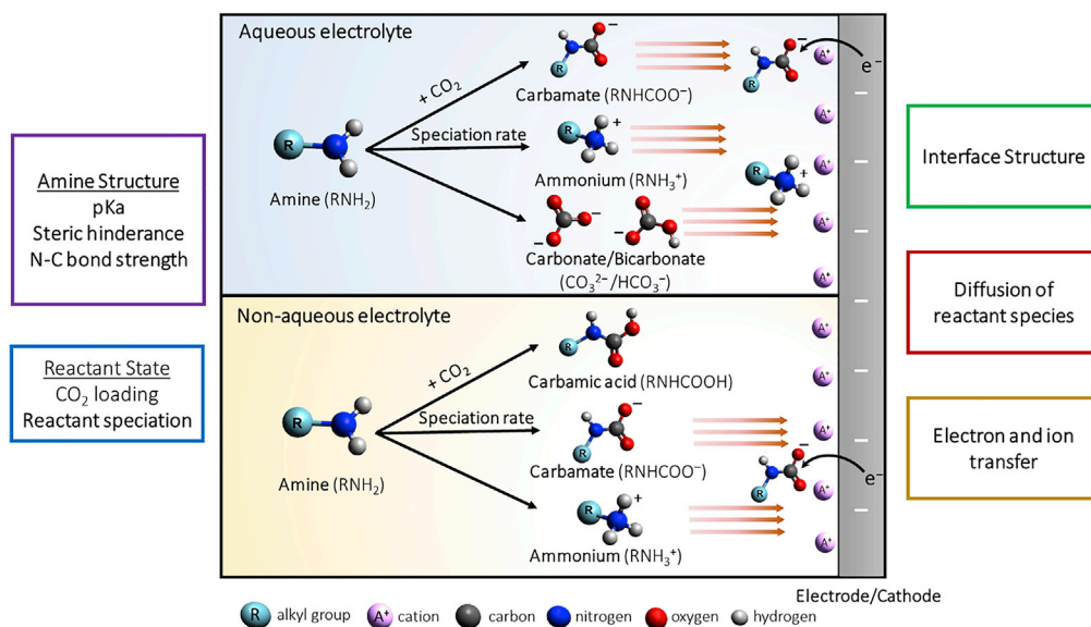
Figure 2. Parameters governing integrated CO 2 capture-electrochemical conversion
