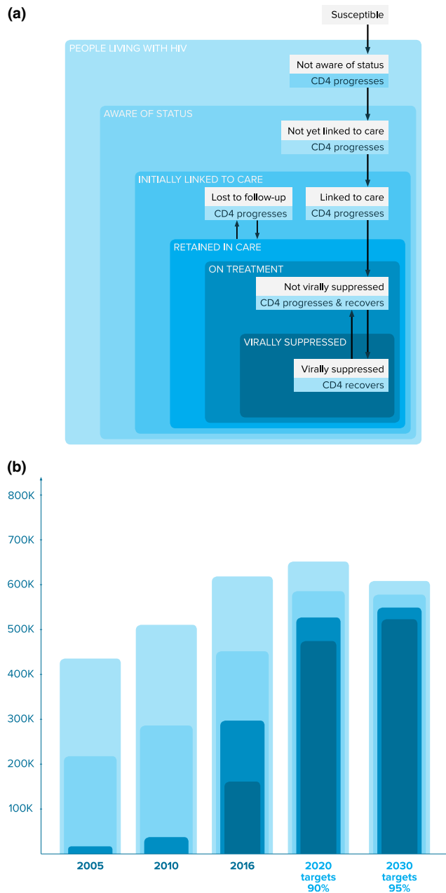
Figure 2. (a) The compartmental structure of the Optima HIV epidemic model, adapted to account for the care and treatment cascade; (b) Progress towards the Fast-Track targets over 2005–2016 (first 3 columns), and model estimates of the scale-up required to 2020 and 2030 (final 2 columns).
