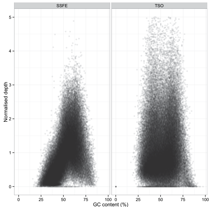
Figure 2. Capture biases for the two kits. The degree of GC bias seen is greater for the SSFE data ( r^2 = 0.56 vs. r^2 = 0.09 for SSFE and TSO respectively, p < 2.2 \times 10^{-16} for both, Pearson's correlation).
