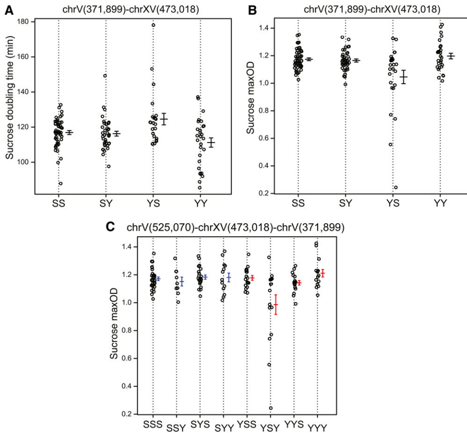
Figure 3 Scatter plots for growth parameters in sucrose showing two-QTL and three-QTL interactions. (A, B) Two-QTL scatter plots for chrV (371,899) and chrXV(473,018) for doubling time and maxOD, respectively. The QTL are indicated as chromosome number followed by marker position in bp within brackets. The x-axis indicates biallelic marker genotype in the QTL order written above the plots. (C) A three-QTL scatter plot for chrV(525,070), chrXV(473,018), and chrV(371,899) for maxOD. The QTL are indicated as chromosome number followed by marker position in bp within brackets. The x-axis indicates triallelic marker genotype in the QTL order written above the plot. The color of error bars ( \pm 1 SE) indicates allele of chrV(525,070) marker with S allele (blue) and Y allele (red).
