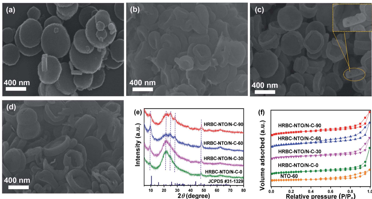
Fig. 3 SEM images of (a) HRBC-NTO/N-C-0, (b) HRBC-NTO/N-C-30, (c) HRBC-NTO/N-C-60, and (d) HRBC-NTO/N-C-90. (e) XRD patterns of HRBC-NTO/N-C-x. (f) N_2 sorption isotherms of HRBC-NTO/N-C-x and NTO-60.
