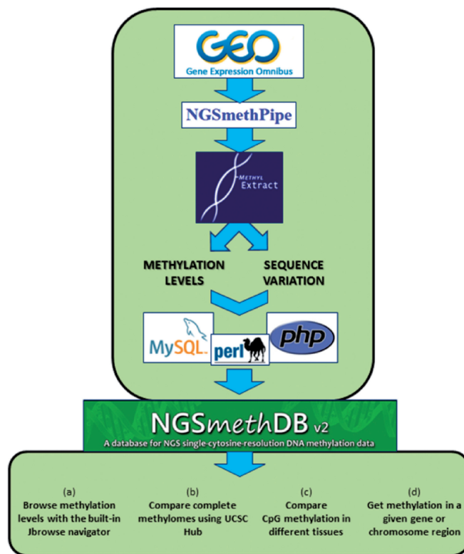
Figure 1. Flow diagram showing the implemented steps and main features of NGSmethDB.
