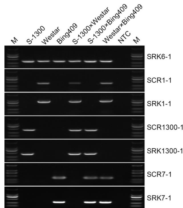
Figure 1. PCR fragment amplified and obtained from three kinds of parent materials and F 1 generation of one-by-one pairs using SCAR markers. NTC: no template control. M: DNA marker, from top to bottom, the size of band was 2000, 1000, 750, 500, 300, and 200 bp, respectively.
