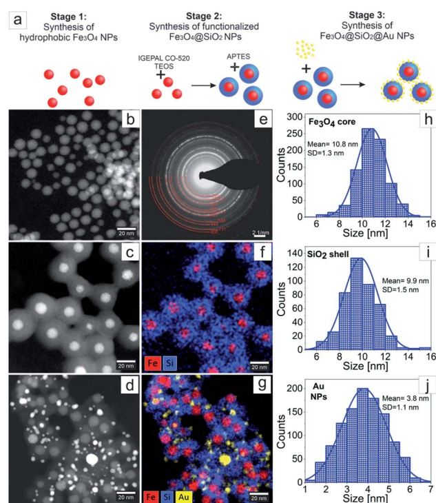
Fig. 2 Schematic diagram of the three stages of \text{Fe}_3\text{O}_4@SiO_2@Au NPs synthesis (a); HAADF STEM overview of \text{Fe}_3\text{O}_4 (b), \text{Fe}_3\text{O}_4@SiO_2 (c) and \text{Fe}_3\text{O}_4@SiO_2@Au NPs; SAED pattern of \text{Fe}_3\text{O}_4 NPs (e); EDX elemental maps of Fe, Si, and Au distribution in \text{Fe}_3\text{O}_4@SiO_2 (f) and \text{Fe}_3\text{O}_4@SiO_2@Au (g) NPs; the distributions of: \text{Fe}_3\text{O}_4 NPs size (h), SiO_2 shell thickness (i) and Au NPs size (j).
