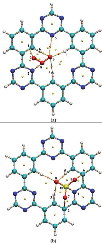
Fig. 5 QAIM analysis results of analytes@CTF-0 complexes i.e. , (a) O_3@CTF-0 complex and (b) SO_3@CTF-0 complex: bond paths are indicated by lines between analyte and CTF-0 surface, whereas bond critical point (BCPs) are indicated by colored dots.
