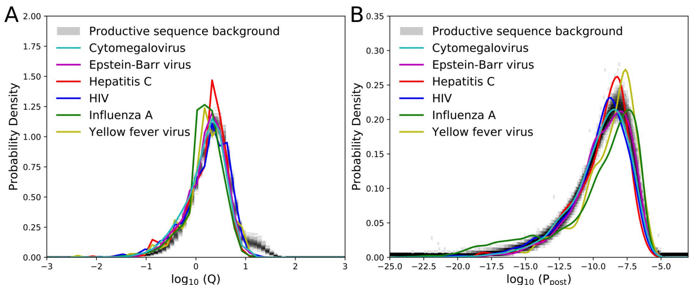
Fig 6. Distribution of TRB sequences from the VDJDdb database specific to human viruses [19] compared to the productive sequences from the blood of 651 individuals. (A) \log_{10}(Q^{\text{univ}}) distribution for each individual's productive data sequences (gray heatmap) and for viral-specific TCRs from the VDJDdb database. (B) \log_{10}(P_{\text{post}}^{\text{univ}}) distributions. The VDJDdb \log_{10}(P_{\text{post}}^{\text{univ}}) distributions are Gaussian-smoothed for clarity. Q^{\text{univ}} and P_{\text{post}}^{\text{univ}} are 'universal' models learned from sequences randomly drawn from all individuals.
