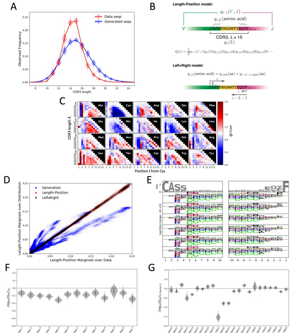
Fig 4. Selection models of 651 individuals. (A) Length distribution of the Complementarity Determining Region 3 (CDR3) of TRB before (as predicted by the P_{gen} model in blue), and after (data, in red) selection. Violin plots show variability across individuals. (B) Illustration of the LengthPosition and Left+Right SONIA models. Both models have the same selection features for gene choice q_{V,J} and CDR3 length q_L . The LengthPosition model has features for amino acid/position/length combinations q_{i,L}(aa) while the Left+Right model factorizes those terms into two terms indexing the amino acid from the left and right edges of the CDR3, i.e. q_{i,L}(aa) = q_{i,left}(aa) \times q_{i-L-1,right}(aa) . (C) Amino-acid selection factors q_{i,L} of the LengthPosition model as a function of position i and L for each of the 20 amino acids. The color scale indicates if a selection factor is above (red) or below (blue) neutral selection. These factors are consistent with previous reports on a smaller cohort [17]. (D) Model prediction for the frequencies of all features of the LengthPosition model ( V,J joint usage, CDR3 length, and amino acid usage at each position and length). The Left+Right model describes the marginals despite not learning them directly. (E) Sequence logos illustrating amino-acid selection factors of the Left+Right model. The first row shows non selected amino acid usage as standard sequence logos while the subsequent rows show right ( \log_{10} q_{i,left}(aa) ) and left ( \log_{10} q_{i,right}(aa) ) for 6 individuals. We include a line for neutral selection, q_i(aa) = 1 , for clarity. (F,G) Distributions of marginal selection factors for J genes and V gene families over the population (calculated by averaging q_{V,J} over the relevant V gene and/or J gene probabilities).
