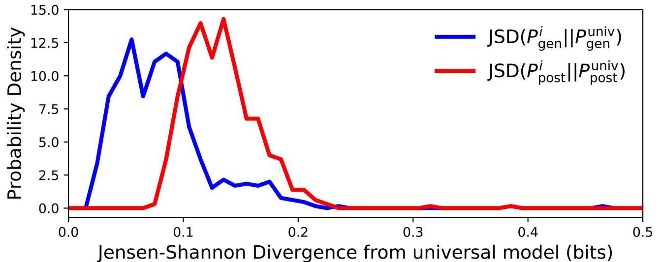
Fig 7. Normalized distributions of the Jensen-Shannon divergence (JSD) of each individual from the universal model for both P_{gen} and P_{post} .
