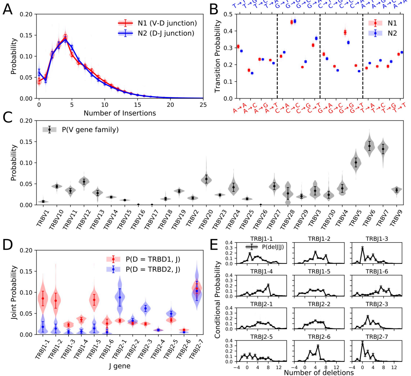
Fig 2. Distribution of the individual P_{gen}^i model parameters over 651 individuals. All plots are violin plots with the mean and standard deviation shown by error bars. (A) Insertion length distributions of the N1 and N2 junctions. (B) Markov transition probabilities for the inserted nucleotide identities at the N1 (red) and N2 (blue) junctions. The N2 transition probabilities are organized in a reverse complementary fashion to the N1 transition probabilities. (C) V gene family usages. (D) Joint D and J gene usages. (E) Deletion profiles for individual J genes. (deletion profiles for the V genes are shown in S1 Fig).
