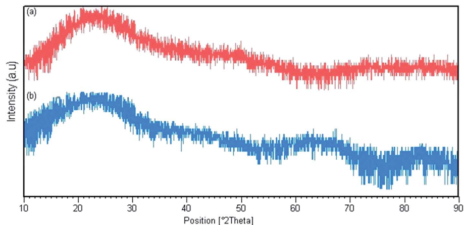
Fig. 3 X-ray diffraction pattern for (a) Pmic11 and (b) Pmic21.
