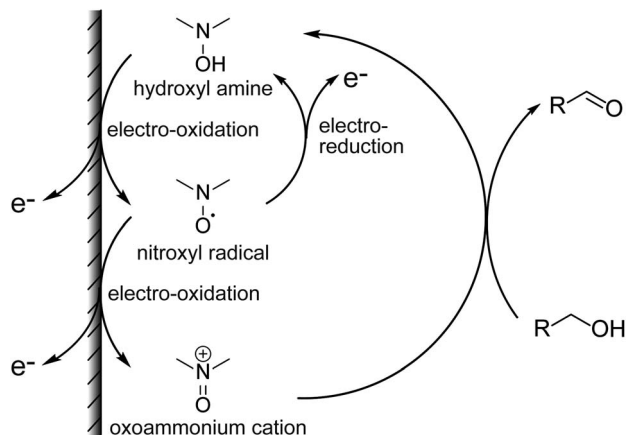
Fig. 1 Electrochemical detection of alcohols using nitroxyl radicals.
