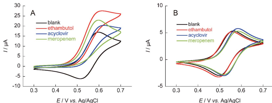
Fig. 4 Cyclic voltammograms of (A) 1 mM NNO and (B) 1 mM TEMPO in the absence and presence of 1 mM ethambutol, acyclovir, and meropenem in 100 mM phosphate buffer (pH 7.4); scan rate: (A) 100 \text{ mV s}^{-1} , (B) 10 \text{ mV s}^{-1} .
