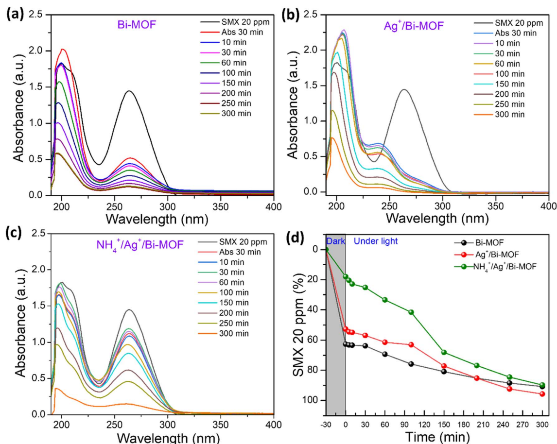
Fig. 5 UV-Vis absorption and photocatalysis of (a) Bi-MOF (pH 6.4), (b) \text{Ag}^+/\text{Bi-MOF} (pH 6.4), and (c) \text{NH}_4^+/\text{Ag}^+/\text{Bi-MOF} (pH 6.0) for the removal of SMX at 27 °C; (d) summary of degradation of SMX under visible light by Bi-MOF, \text{Ag}^+/\text{Bi-MOF} , \text{NH}_4^+/\text{Ag}^+/\text{Bi-MOF} .
