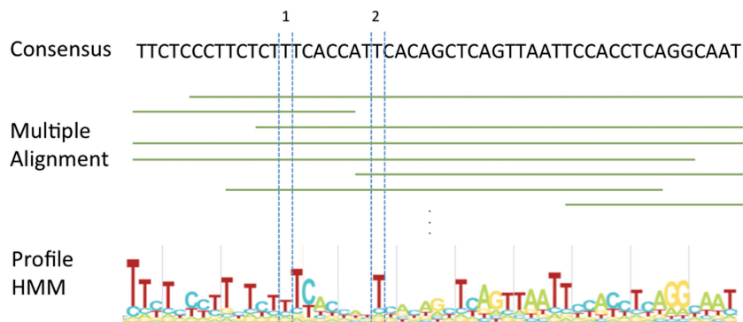
Figure 2. Schematic representation of the creation of the multiple sequence alignment and profile HMM for a Dfam entry. The consensus and HMM logo correspond to positions 253–304 of Tigger16a (DF0000028), and highlight the difference between the abilities of HMM and consensus to represent positional residue conservation — a consensus treats all majority rule decisions as equivalent, while a profile HMM enables position-specific scoring based on conservation. In this case, the position labelled with (1) has a slight preference for ‘T’, but will not substantially reward a ‘T’ or penalize any other nucleotide; meanwhile the position labelled with (2) shows a strong preference for ‘T’, and will provide high reward for a matching ‘T’, and a strong penalty for any other nucleotide.
