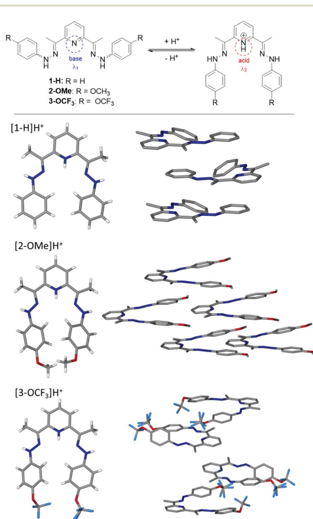
Fig. 1 Compounds 1–3 and their proposed behaviour in acid–base media (top). Crystal structures of the protonated compounds 1–3 and their crystal packing arrangement (presented with non-hydrogen atoms displayed): [1-H]H + ; [2-OMe]H + ; [3-OCF 3 ]H + (bottom).
