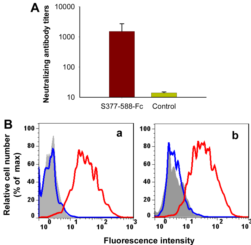
Figure 5. Detection of neutralizing antibodies in S377-588-Fc protein-vaccinated mouse sera and antibody-mediated blockage of receptor binding. (A) Sera collected at 10 days post-last vaccination were tested for neutralization of MERS-CoV infection in Vero E6 cells. PBS was used as the control. Neutralizing antibody titers were expressed as the reciprocal of the highest dilution of serum that completely inhibited virus-induced CPE in at least 50% of the wells ( NT_{50} ), and the results are presented as mean \pm SD from five mice per group. (B) Collected mouse sera were tested for blockage of S377-588-Fc binding to DPP4-expressing Huh-7 cells by flow cytometry. (a) The S377-588-Fc protein (red line) bound efficiently to Huh-7 cells (gray shade), while only background binding was shown in the control protein hlgG-Fc (blue line). (b) Blockage of S377-588 binding to Huh-7 cells (gray shade) by vaccinated mouse antisera (1:32, blue line). Sera from the PBS control group (red line) were included as the control. doi:10.1371/journal.pone.0081587.g005
