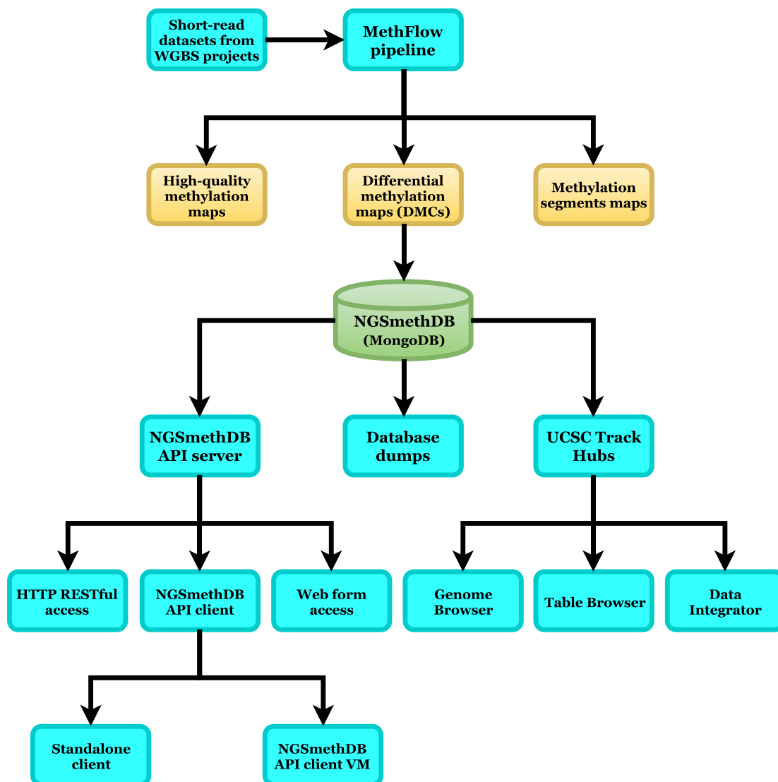
Figure 1. Data flow diagram for NGSmethDB indicating the source of primary data, the different types of extracted data and the different ways of data access.
