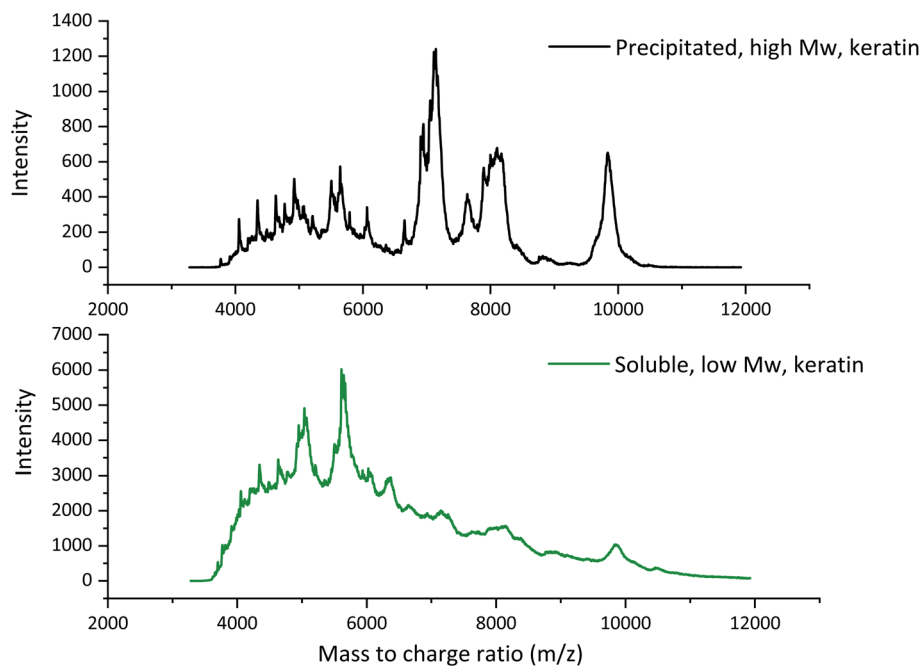
Fig. 2 The MALDI-TOF spectra of high M_w and low M_w keratin fractions.
