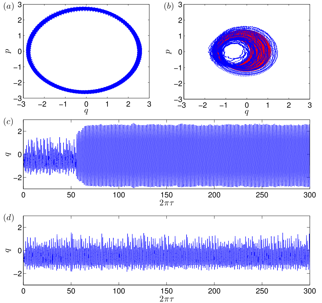
Figure 3. For g_0/\omega_m=0.1 , (a) an asymptotic quantum trajectory calculated from the QSD method, (b) the quantum trajectory in the transient phase, overlapped with the corresponding classical trajectory, (c) the corresponding time series. The asymptotic quantum trajectory is regular, in spite of the quantum fluctuations. However, the transient quantum trajectory is chaotic and coincides well with the classical trajectory (gray). (d) An example of a very long chaotic transient in the quantum regime for g_0/\omega_m=0.05 .
