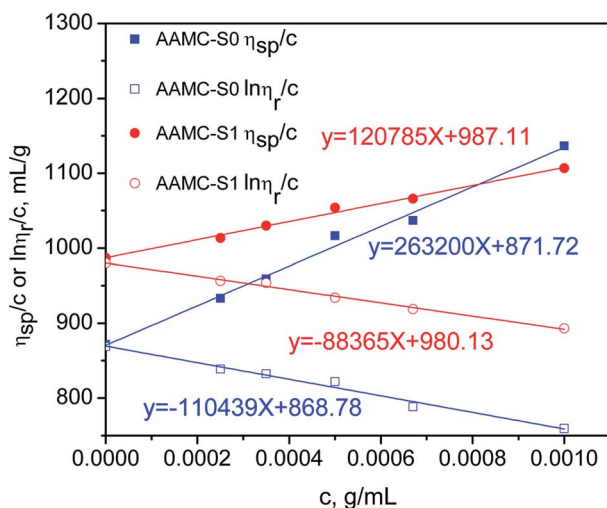
Fig. 8 Relationship between \eta_{sp}/c ( \ln \eta_r/c ) and concentration of samples.
