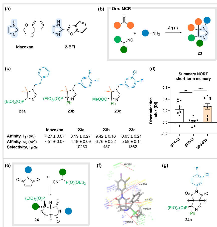
Figure 9. I_2 Imidazoline receptors. (a) Structure of known I_2 IR ligands. (b) MCR access to substituted 2-imidazolines 23 . (c) Structure and binding affinities of the selected compounds. (d) In vivo data of compound 23b . (e) Condensation between maleimides and PhosMIC derivatives leading to new I_2 -IR ligands 24 . (f) 3D-QSAR series 24 . (g) Structure of the selected analogue 24a . Values represented in (d) are mean ± Standard error of the mean (SEM); n = 36 (SR1-Ct n = 11; SP8-Ct n = 11; SP8-23b n = 14). ** p < 0.01 ; *** p < 0.001 .
