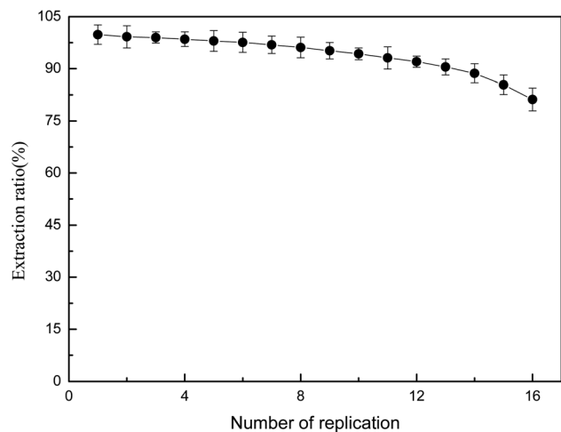
Fig. 6 Reusability of PILs-C 5 .
