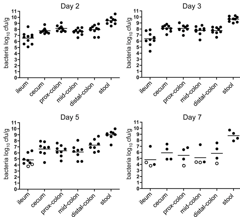
Figure 2. Kinetics of C227 colonization in infant rabbits
