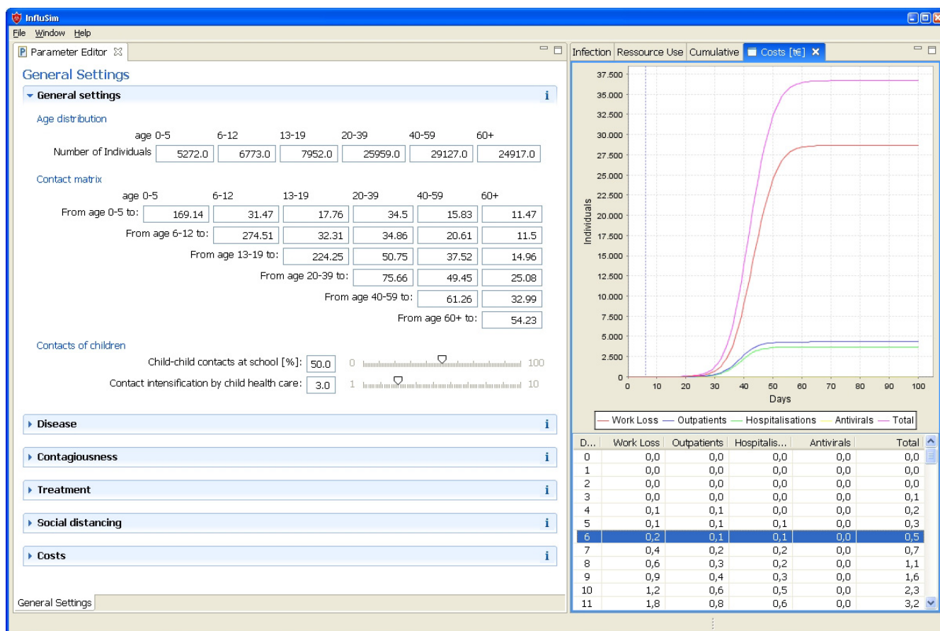
Figure 1 InfluSim user interface. Graphical user interface of InfluSim . Parameter values can be varied within different tabs (left hand side), divided into General settings (demography by age and risk group, contact matrix, economics), Disease (sojourn times, symptoms, hospitalizations, case fatality), Contagiousness ( R_0 , infectivity over time and by disease severity), Treatment (therapeutic window, treatment schedules, antiviral properties), Social distancing (isolation schedules, general contact reduction, closing day care centres and schools, cancelling mass gatherings) and Costs (work loss, hospitalization, treatment). Time-dependent model output (right hand side) visualizes Infection prevalence (susceptible, exposed, asymptomatic, moderately sick, severely sick, dead, immune), Resource use (work loss, outpatients, hospital beds, antivirals), Cumulative numbers of the latter, and Costs .
