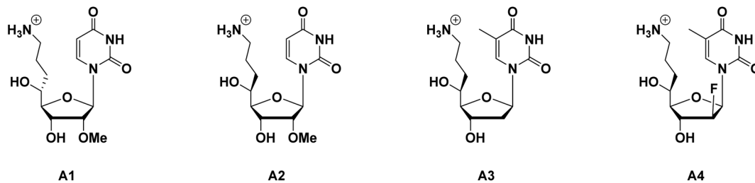
Fig. 1 The chemical structure of ( R )-5'-aminopropyl-2'-OMe-uridine (A1), ( S )-5'-aminopropyl-2'-OMe-uridine (A2), ( S )-5'-C-aminopropyl-thymidine (A3) and ( S )-5'-C-aminopropyl-2'- \beta -fluoro-thymidine (A4).
