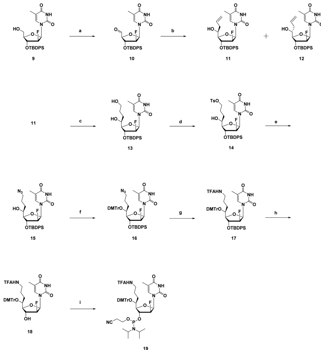
Scheme 2 Synthetic route of ( S )-5'- C -aminopropyl-2'-β-fluoro-thymidine phosphoramidite 19 . 9 Reagents and conditions: (a) EDC·HCl, CHCl 2 CO 2 H, DMSO/DCM (1 : 1 v/v), 0 °C, 3 h; (b) allyltrimethylsilane, BF 3 ·Et 2 O, DCM, 0 °C, 3 h; 11 : 71% (2 steps); 12 : 4% (2 steps); (c) (1) 9-BBN, THF, r.t., over-night; (2) 2 N NaOH aq., 30% H 2 O 2 aq., r.t., 15 min; 13 : 77%; (d) p -TsCl, Me 2 N(CH 2 ) 3 NMe 2 , DCM, -10 °C, 2 h; 14 : 81%; (e) NaN 3 , DMF, 60 °C, over-night; 15 : 76%; (f) DMTrOTFA, DIPEA, THF, r.t., 22–24 h; 16 : 93%; (g) (1) Ph 3 P, H 2 O, THF, 40 °C, 24 h; (2) CF 3 CO 2 Et, Et 3 N, DCM, r.t., over-night; 17 : 96%; (h) TBAF/THF, THF, r.t., 2 h; 18 : 95%; (i) DIPEA, CEPL, THF, r.t., 1.5 h; 19 : 89%.
