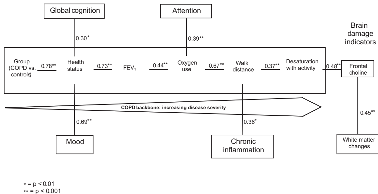
Figure 1 Modeling the impact of COPD on brain function ( R^2 shown).
