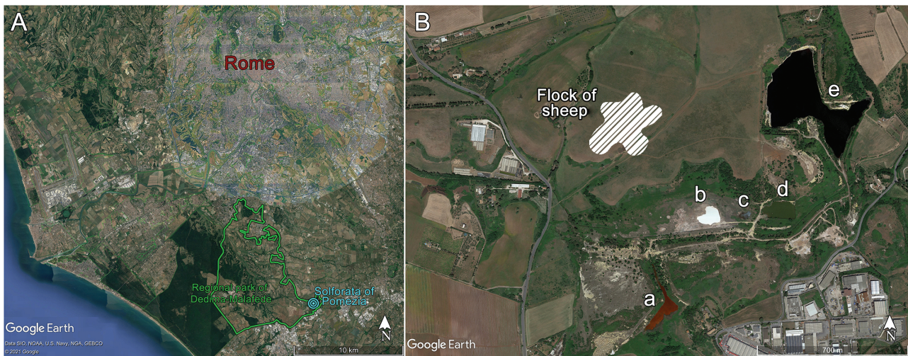
Fig. 1. Satellite imagery. In (A) the regional park of Decima-Malafede, southern of Rome, with highlighted the location of Solfiorata (bottom right circle); in (B), identified by lower case letters, the five WBs present in the Solfiorata area: the red lake and the white lake ( WB_a and WB_b ), two small lakes ( WB_c and WB_d ), and the inundated basin of the old mining zone ( WB_e ). See Carapezza et al. (2012) for the CO_2 and H_2S soil flux maps of the area.
