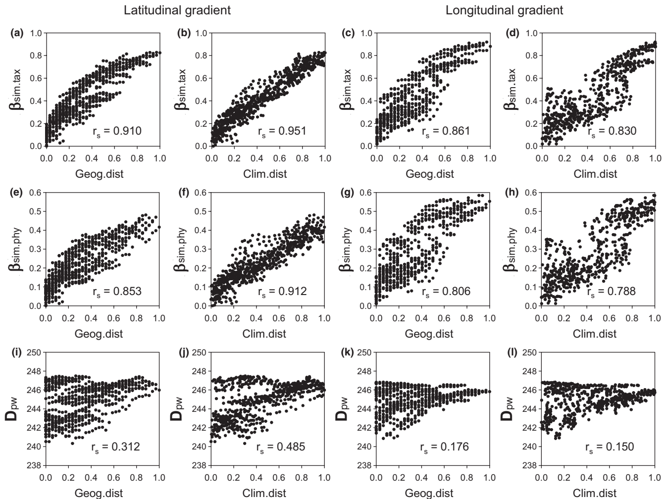
FIGURE 1 Relationships of taxonomic and phylogenetic \beta -diversity ( \beta_{\text{sim.tax}} , \beta_{\text{sim.phy}} , and D_{\text{pw}} ) with geographic distance (Geog.dist) and climatic distance (Clim.dist) for angiosperms in sites of 100 km \times 300 km along latitudinal and longitudinal transects in China (see Appendix S1 for details about the two transects). Geographic and climate distances were rescaled to vary between 0 and 1 within each transect
