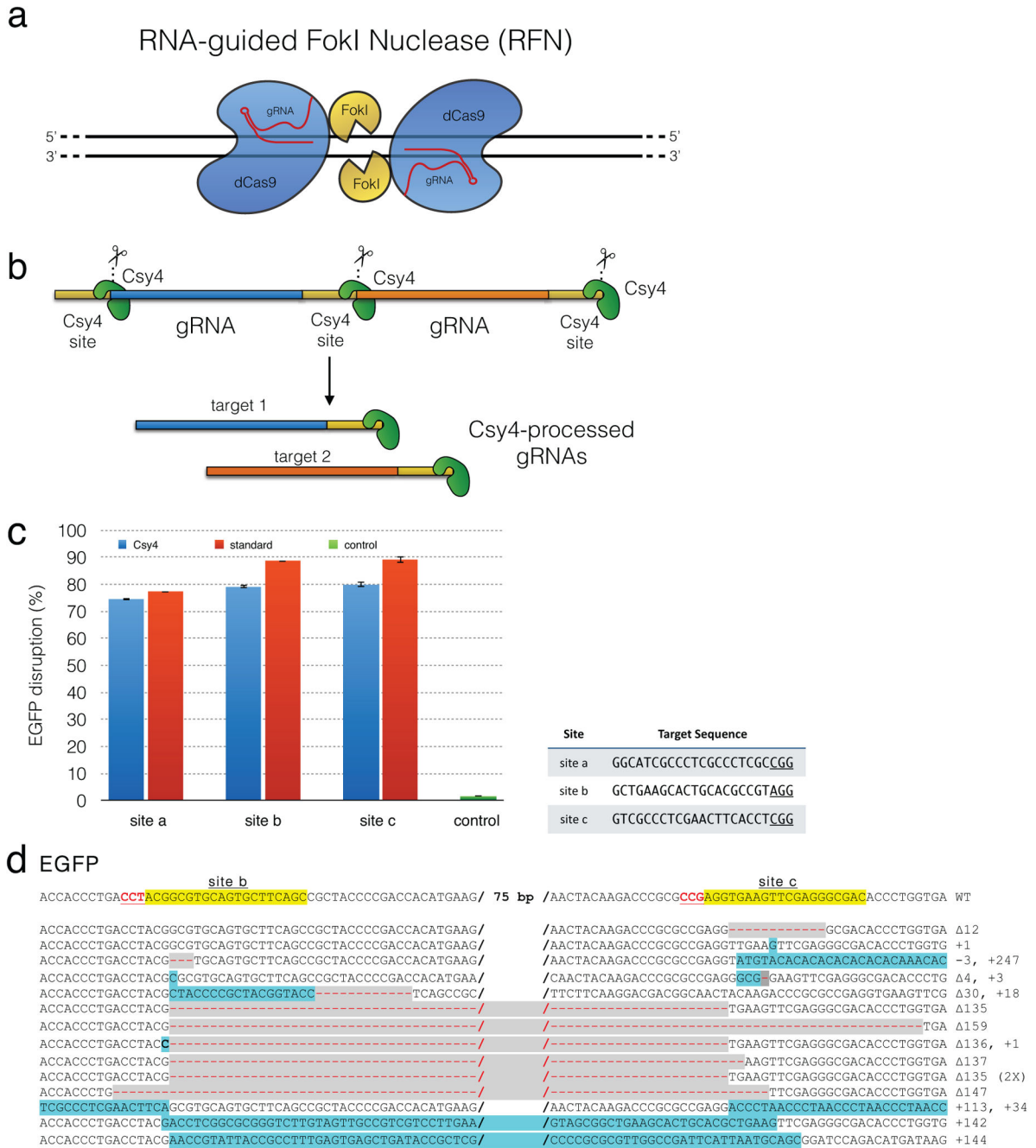
Figure 1. RNA-guided FokI nucleases and a Csy4-based multiplex gRNA expression system (a) Schematic overview of RNA-guided FokI nucleases. Two FokI-dCas9 fusion proteins are recruited to adjacent target sites by two different gRNAs in order to facilitate FokI dimerization and DNA cleavage. (b) Schematic overview of a Csy4-based multiplex gRNA expression system. Two gRNAs (with any 5' end nucleotide) are co-expressed in a single transcript from a U6 promoter with each gRNA flanked by Csy4 recognition sites. Csy4 cleaves and releases gRNAs from the
