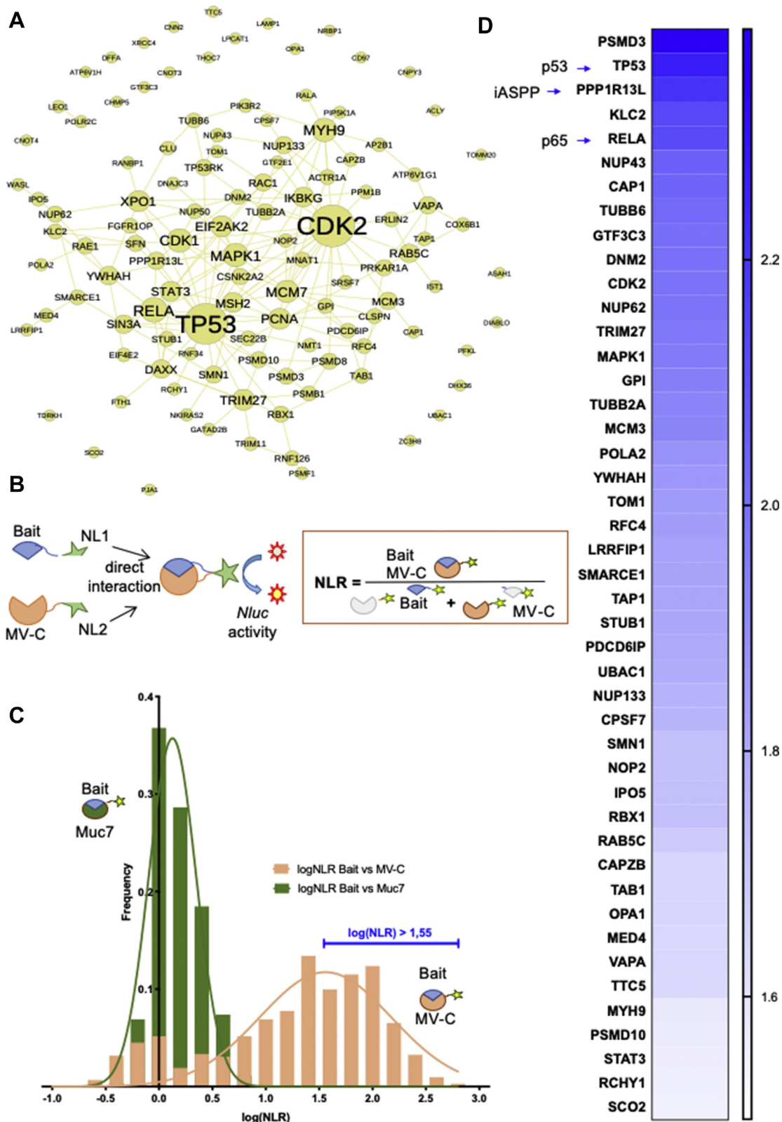
FIG. 5. Protein complementation assay (PCA) for MV-C protein and 119 host-interacting proteins. A , representation of the PPI network selected for PCA. Gephi 0.9.2 was used to represent the PPI network. B , schematic representation of PCA approach. A host protein (prey) is fused downstream to the N-half of the Nluc (NL1). MV-C (bait) is fused downstream to the C-half of the Nluc (NL2). The formula to calculate normalized luminescence ratio (NLR) for a given protein pair is shown. C , frequency distribution of log(NLR) values for the MV-C and the Muc7
