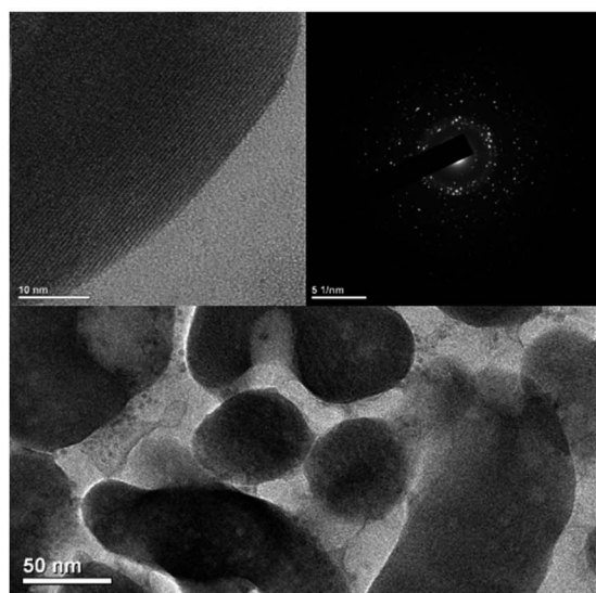
Fig. 7 TEM images of (a) as-quenched glass and (b) partially crystallized sample, and the corresponding SAED pattern with the scale bar of 5 \text{nm}^{-1} in the inset of each figure, a grain boundary of nanocrystal is shown in the inset of (b) with the scale bar 10 nm.
