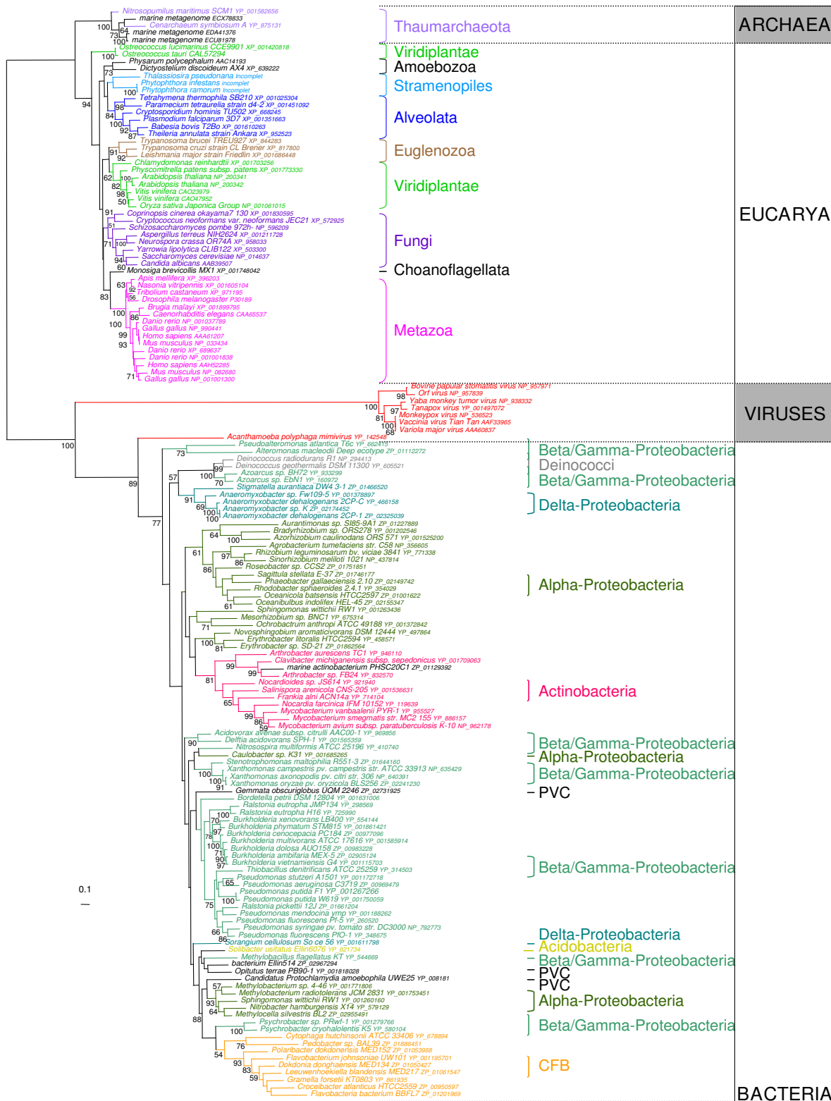
Figure 2 Unrooted maximum likelihood phylogenetic tree of 151 Topo IB sequences. Numbers at branches represent bootstrap proportions. The scale bar represents the average number of substitutions per site.
