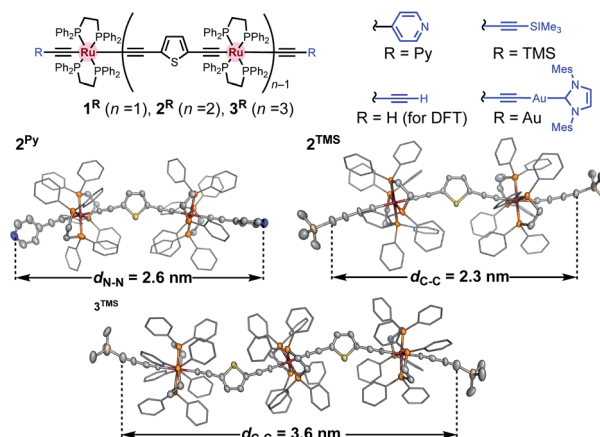
Fig. 3 Molecular structures of n^R ( n = 1-3 ; R = \text{Py} , \text{H} , \text{TMS} , and \text{Au} ) and X-ray structures of 2^{\text{Py}} , 2^{\text{TMS}} , and 3^{\text{TMS}} . Thermal ellipsoid plots are set at the 50% probability level. Phenyl rings are represented by a stick model. Hydrogen atoms, solvent molecules, and disordered parts are omitted for clarity.
