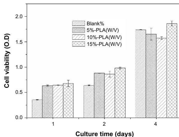
Figure 7 NIH3T3s proliferation on porous PLA scaffolds. The number of cells was normalized to initial density of seeded cells ( 1 \times 10^5 cells/well). Mean for n = 3 \pm SD .
