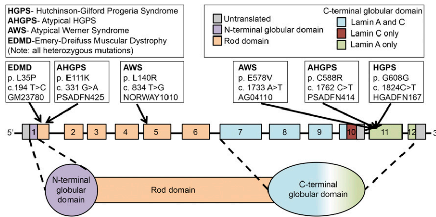
Fig. 1. Diagram of the locations of LMNA mutations in the cell lines used in this study. Each putative causative mutation is indicated along with the name of the cell line that harbors it and the disease it causes. The top left key shows the name of each disorder, and the top right key shows the color code for the domains of lamin A and/or C. The LMNA gene is not drawn to scale. Adapted with permission from ref. 7.
