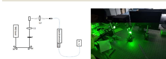
Fig. 1 Raman device diagram.
