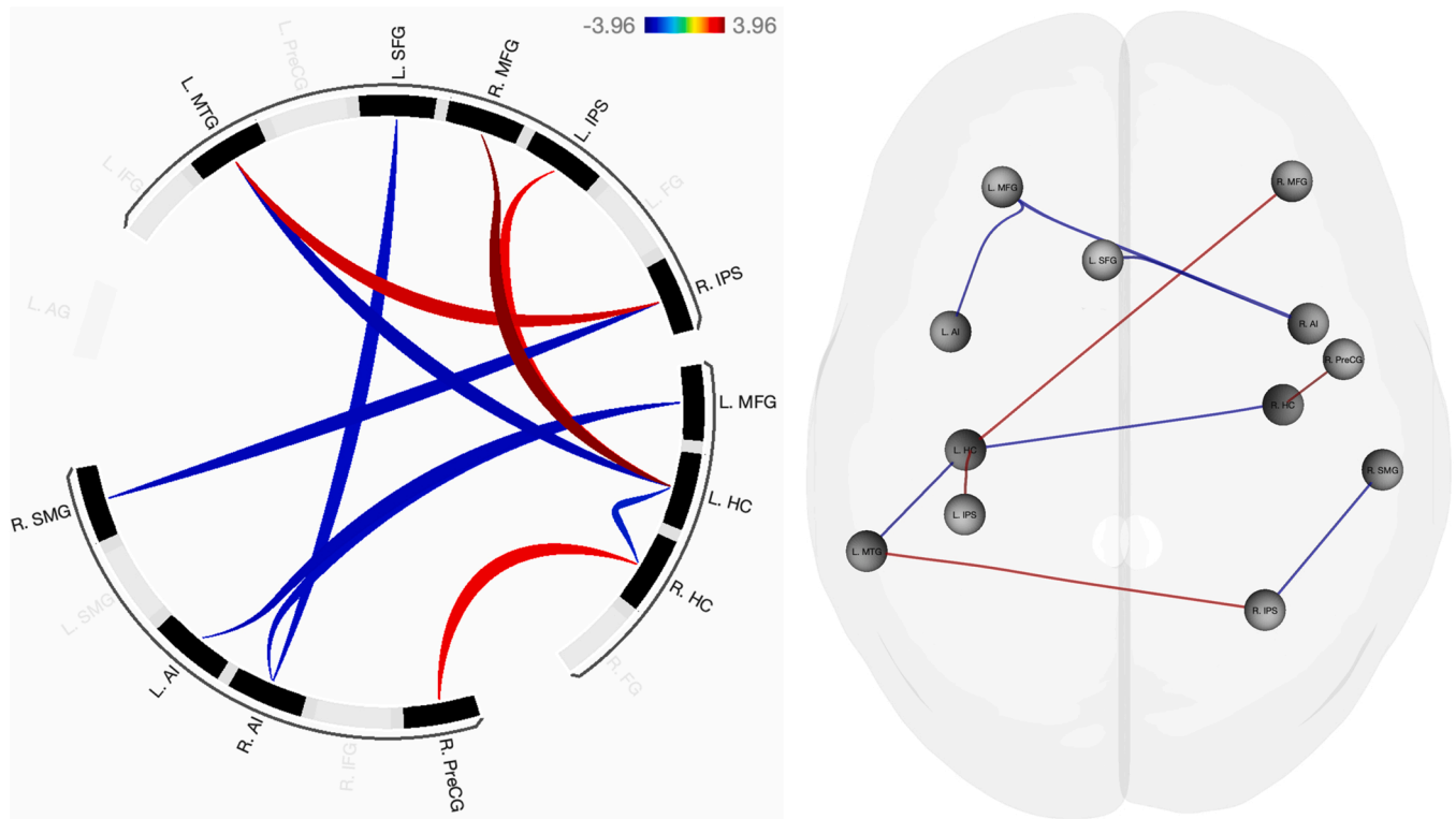
Fig. 3. Functional connectivity differences associated with verbal number comparison, controlled for general decision-making ability. Blue: increased FC negatively associated with age; red: increased FC positively associated with age.
