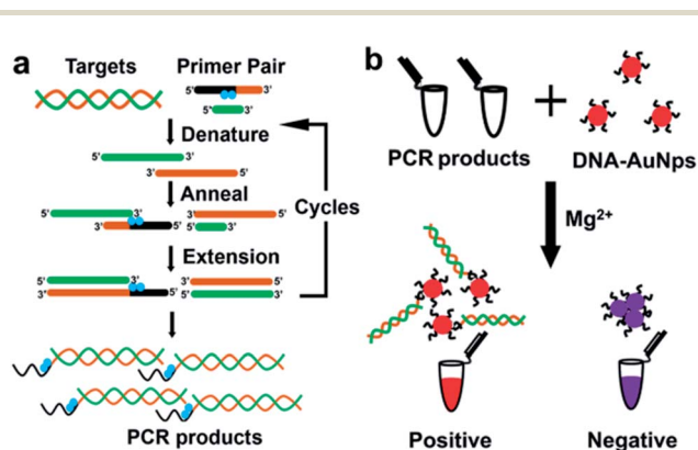
Scheme 1 Outline of the visual detection of designated gene proposed in this paper. In the “indenting PCR” (a), PCR products having an overhang are prepared by placing multiple “molecular blockers” (blue circles) in tandem in one of the primers. In (b), these PCR products are treated with AuNps, labelled with the probe oligonucleotide, in the presence of appropriate concentration of Mg^{2+} . The overhang having complementary sequence, if any, should bind to the probe DNA on the AuNps and prevent the particles from aggregation (the left in (b)). Otherwise, the salt-induced aggregation promptly occurs (the right). Thus, the presence or the absence of the designated gene in the original specimen is differentiated simply in terms of the color of the solution (either red or blue).
