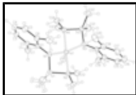
Fig. 1. The molecular structure, showing the atom-numbering scheme. Displacement ellipsoids are drawn at the 30% probability level. H atoms are presented as a small spheres of arbitrary radius.
