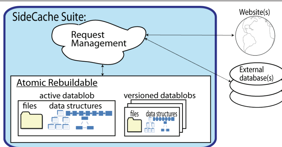
Figure 2 The atomic rebuildable data blob.
