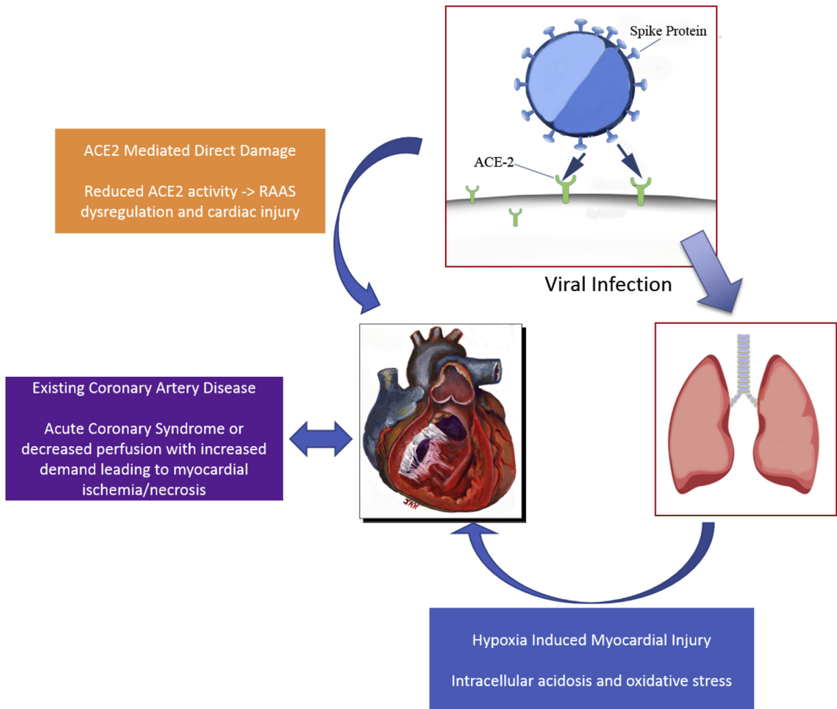
Fig. 1. Possible mechanisms of cardiac injury with COVID-19.
