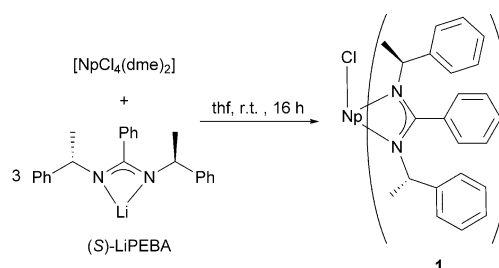
Scheme 1. Synthesis of the \text{Np}^{\text{IV}} amidinate [\text{NpCl}((S)\text{-PEBA})_3] 1 .
