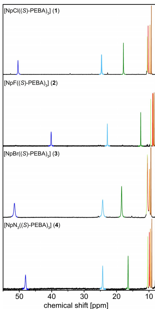
Figure 2. Part of ^1\text{H} NMR spectra of [\text{NpX}((\text{S})\text{-PEBA})_3] ( \text{X} = \text{Cl} (1), F (2), Br (3), \text{N}_3 (4)). Similar protons are colored with similar colors (blue/pale blue: NC-H; green/pale-green: ortho -Ph; red/orange: meta -Ph, brown: para -Ph).
