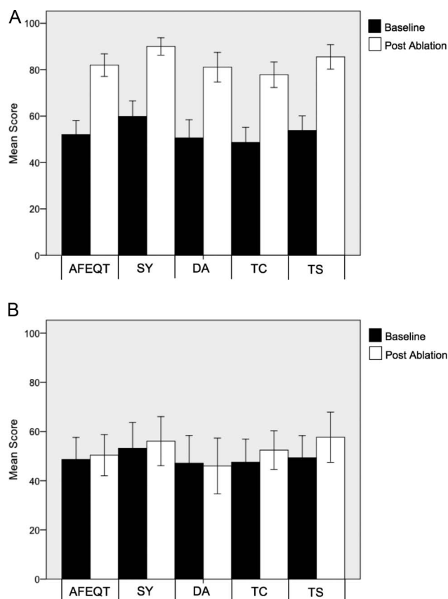
Figure 1 Mean individual and summative AFEQT scores before and 3 months after ablation. (A) Patients who maintained sinus rhythm post ablation; (B) Patients with recurrent AF. AFEQT, Atrial Fibrillation Effect on Quality-of-Life; DA, daily activities; SY, symptoms; TC, treatment concern; TS, treatment satisfaction.
