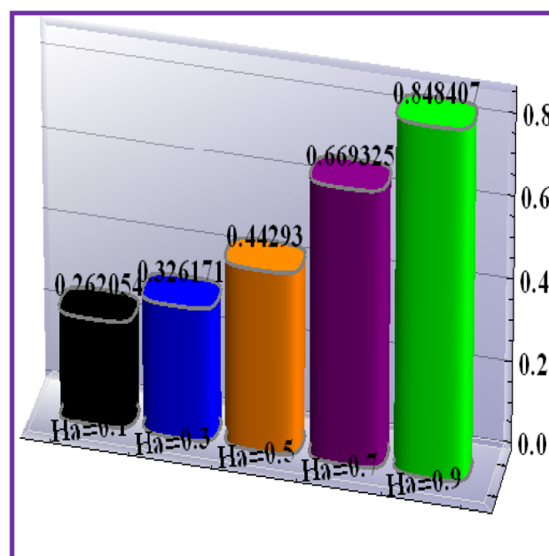
Fig. 19 \frac{1}{2} \text{Re}_x^{1/2} C_f via Ha.
