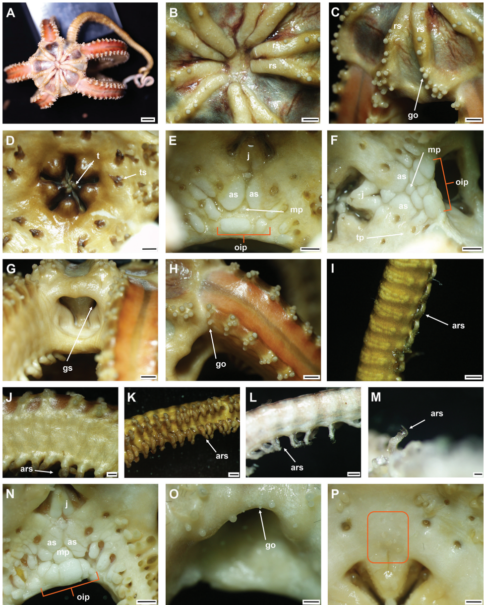
Figure 18. Asterostegus maini McKnight, 2003 (A–M IDSSE-EEB-SW0076 N–P IDSSE-EEB-SW0075) A dorsal view B center of dorsal disc C dorsal disc (distal end of radial shields) D ventral disc E, F oral frame G lateral disc H dorsal arm (proximal) I dorsal arm (distal) J lateral arm (proximal) K ventral arm (middle) L, M arm spines (distal) N oral frame O periphery of the disc P oral frame (small transparent ossicles). Abbreviations: as adoral shield, ars arm spine, go granular ossicle, gs genital slit, j jaw, mp median plate, oip oral interradial plate, rs radial shield, t teeth, tp tentacle pore, ts tentacle scale. Scale bars: 6 mm ( A ); 2 mm ( B–H, N ); 1 mm ( I–K, O, P ); 500 \mu m ( L ); 200 \mu m ( M ).
