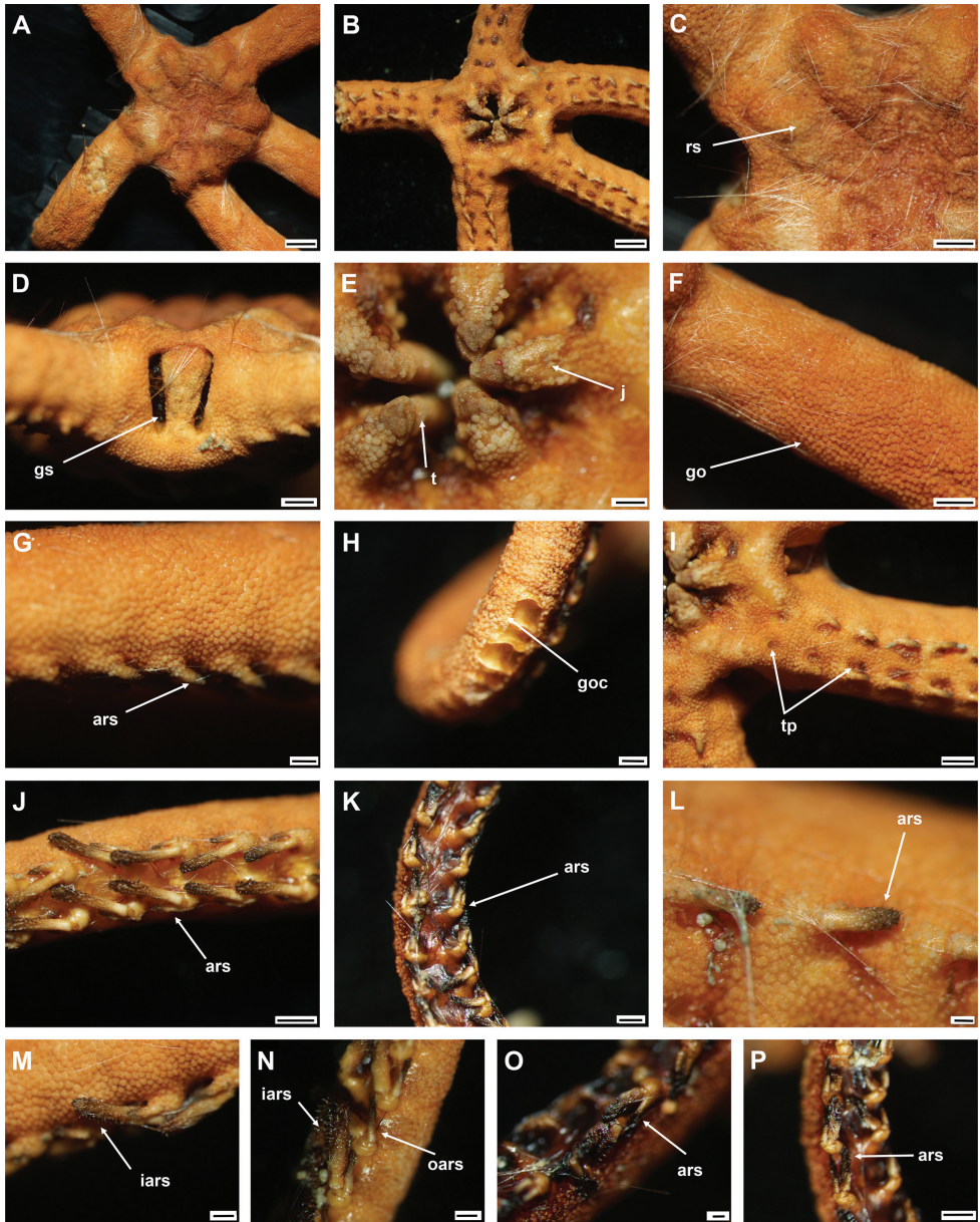
Figure 6. Asterschema shenhaiyongshii sp. nov., holotype (IDSSE-EEB-SW0086) A dorsal view B ventral view C dorsal disc D lateral disc E oral frame F dorsal arm (base) G lateral arm (proximal) H dorsal arm (distal) I ventral arm (base) J ventral arm (middle) K ventral arm (distal) L arm spine (arm base) M , N arm spines (middle) O , P arm spines (distal). Abbreviations: ars arm spine, go granular ossicle, goc granular ossicles coat, gs genital slit, iars inner arm spine, j jaw, oars outer arm spine, rs radial shield, t teeth, tp tentacle pore. Scale bars: 2 mm ( A , B ); 1 mm ( C , D , F , I , J ); 500 \mu m ( E , G , H , K , M , N , P ); 200 \mu m ( L , O ).
