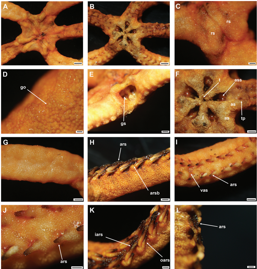
Figure 10. Asterschema rubrum Lyman, 1879 (IDSSE-EEB-SW0072) A dorsal view B ventral view C dorsal disc D skin on the disc E lateral disc F ventral disc G dorsal arm (proximal) H lateral arm (middle) I ventral arm (proximal) J outer arm spine (proximal) K arm spines (middle) L arm spines (distal). Abbreviations: as adoral shield, ass adoral shield spine, ars arm spine, go granular ossicle, gs genital slit, ias inner arm spine, j jaw, oars outer arm spine, ass adoral shield spine, rs radial shield, t teeth, tp tentacle pore. Scale bars: 2 mm ( A, B ); 1 mm ( E–G, I ); 500 \mu m ( C, H, J, K ); 200 \mu m ( D, L ).
