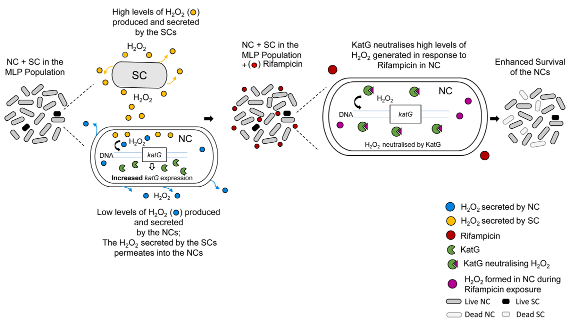
Fig. 9. Model depicting the SCs priming the NCs to enhance their survival against the endogenous H 2 O 2 generated in response to rifampicin. The SCs release high levels of H 2 O 2 which significantly increase katG expression in the NCs co-existing with the SCs at 9:1 ratio in the MLP population. Upon exposure to rifampicin, the H 2 O 2 generated in the NCs in response to rifampicin gets neutralised by the KatG resulting in the enhanced survival of the NCs against rifampicin. The SCs and the NCs are not drawn to the 1:9 proportion indicated in the data due to space constraints.
