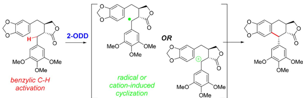
Fig. 72 Mechanism of nonheme iron enzyme 2-ODD catalyzed oxidative cyclization [Reprinted with permission from ref. 53 Copyright 2019 American Chemical Society].
