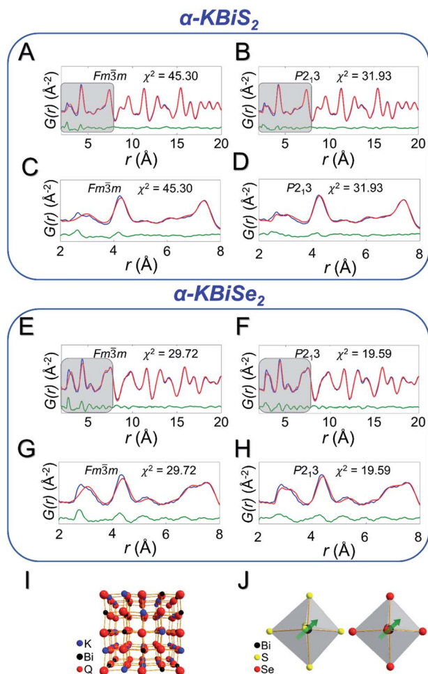
Fig. 6 PDF fits for \alpha - \text{KBiS}_2 using a (A) Fm\bar{3}m model and (B) P2_13 model. These models are zoomed in to the short range ( r < 8 Å), highlighted in grey, for the Fm\bar{3}m model (C) and for the P2_13 model (D). In the PDF fits, red is the calculated PDF pattern, blue is the experimental data, and green is the difference pattern. PDF fits for \alpha - \text{KBiSe}_2 using a (E) Fm\bar{3}m model and (F) P2_13 model; zoomed in region shown for the Fm\bar{3}m model (G) and for the P2_13 model (H). (I) Shows a 2 \times 2 \times 2 unit cell representation of \text{KBiQ}_2 and (J) highlights the off-centering of bismuth in the [\text{BiS}_6]^{3-} and [\text{BiSe}_6]^{3-} octahedra.
