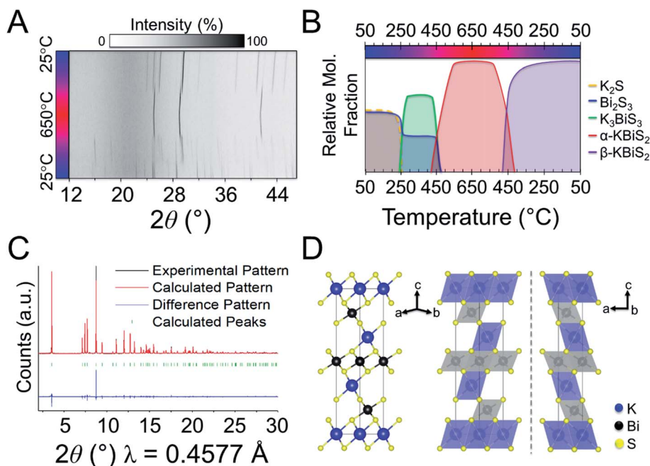
Fig. 4 (A) Overlaid diffraction patterns of 1 \text{K}_2\text{S} + 1 \text{Bi}_2\text{S}_3 . (B) Reaction map of 1 \text{K}_2\text{S} + 1 \text{Bi}_2\text{S}_3 . Nominal compositions are shown; dashed lines represent a noncrystalline phase. (C) Structure solution for \beta\text{-KBiS}_2 . (D) Structural representation of the ordered rocksalt, \beta\text{-KBiS}_2 .
