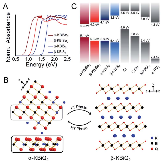
Fig. 7 (A) Experimental band gaps for the known \alpha - \text{KBiQ}_2 ( Fm\bar{3}m ) and discovered \beta - \text{KBiQ}_2 phases ( R\bar{3}m ). (B) Illustration of dimension reduction from the 3D covalent framework in the high temperature (HT) phase, \alpha - \text{KBiQ}_2 , to the layered 2D covalent framework in the low temperature (LT) phase, \beta - \text{KBiQ}_2 . For both structures, only covalent bonds (e.g. Bi–Q bonds) are shown. The site distribution of bismuth and potassium in \alpha - \text{KBiQ}_2 was randomized, while constrained to maintain equivalent amounts of the cations. The inset for \alpha - \text{KBiQ}_2 tilts the indicated portion of the structure to highlight the 3D connectivity through the plane. (C) Depiction of valence band maxima, conduction band minima, and band gap energies for \alpha - \text{KBiQ}_2 , \beta - \text{KBiQ}_2 , Si, 90,91 CdTe, 92 \text{MAPbI}_3 , 93 and \text{TiO}_2 (anatase). 94,95
