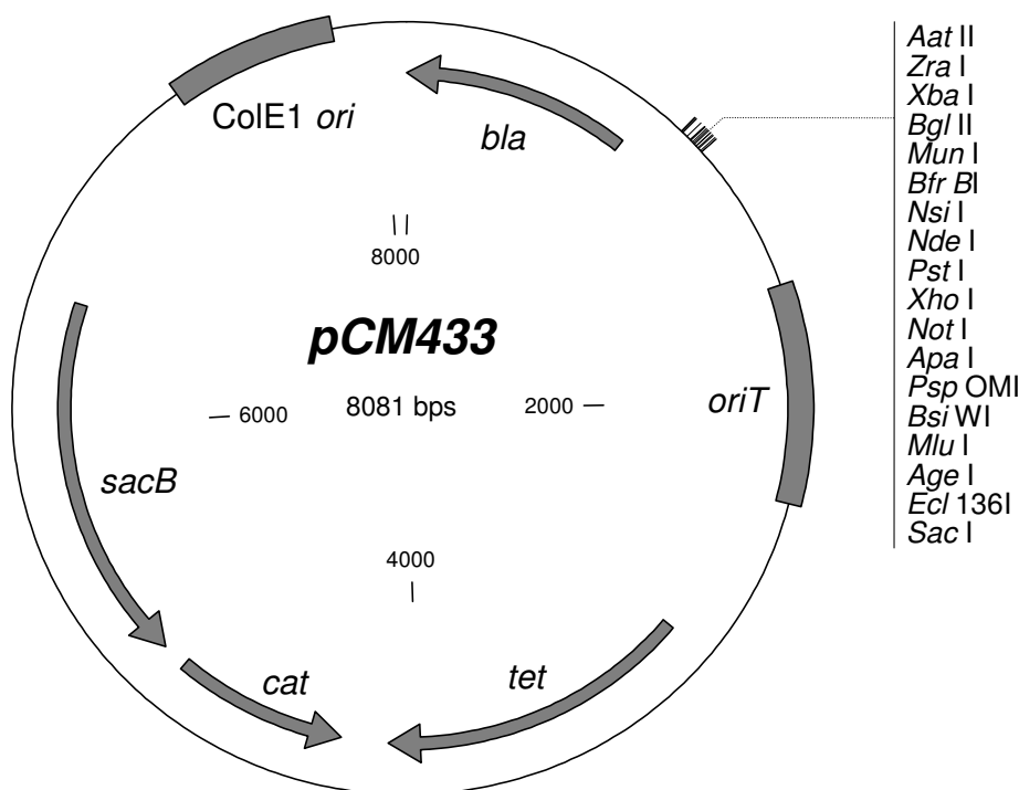
Figure 2 Broad-host-range allelic exchange vector pCM433. Plasmid map of pCM433 [GenBank:EU118176] indicating the available restriction sites in the multiple-cloning site, as well as key plasmid features: bla (encodes beta-lactamase; Ap R ), oriT (IncP origin of conjugal transfer), tet (encodes Tc efflux pump), cat (encodes Cm acetyltransferase), sacB (levansucrase; confers sucrose sensitivity), and ColE1 ori (high copy E. coli origin of replication). Plasmid map was generated using Clone Manager 7 (Sci Ed Central).
